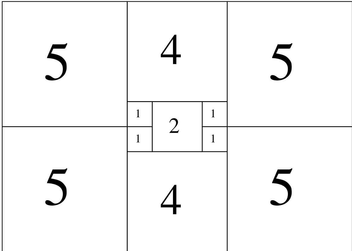
11 : 14 x 10 Octahedron/Cube (1/1)
