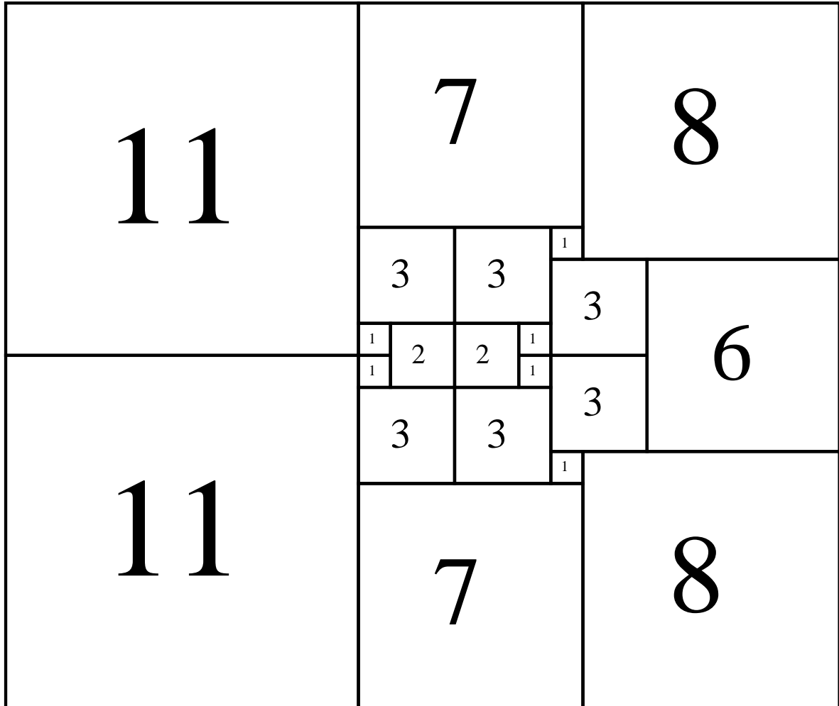
21 : 26 x 22 Cuboctahedron (1/1)
