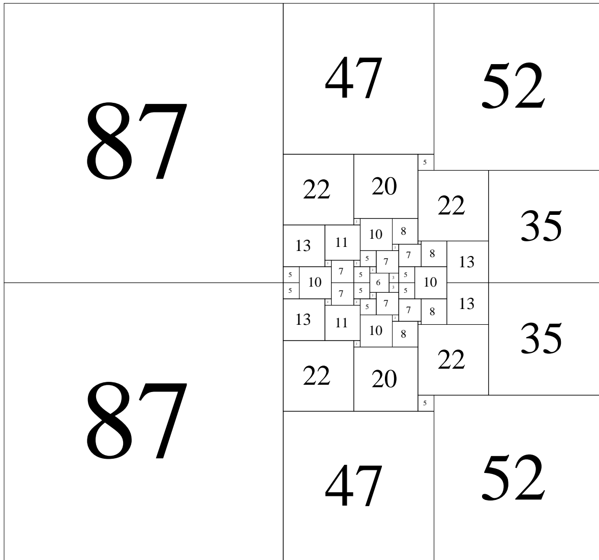
59 : 186 x 174 Icosidodecahedron (1/1)
