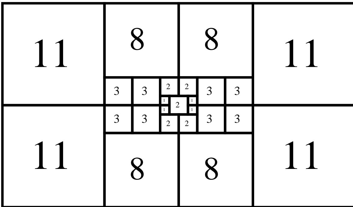
25 : 38 x 22 Icosahedron/Dodecahedron (1/1)
